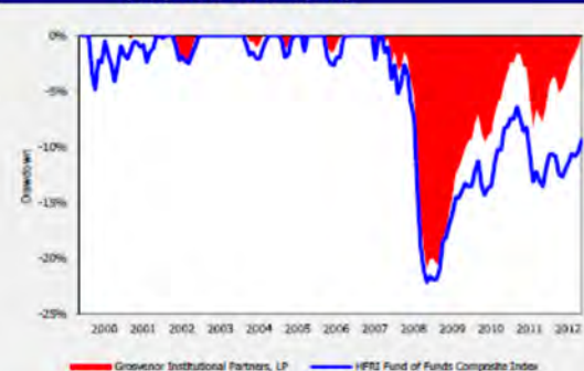
Underwater Drawdowns
